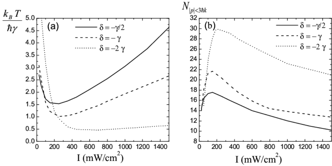
Figure 2. Laser cooling temperature of ^{24}\text{Mg} atoms in \sigma_+-\sigma_- field configuration (a) and fraction of cold atoms (b) as function of intensity of light waves. k_B T/\hbar \gamma = 1 corresponds to T \approx 1.28 mK.
