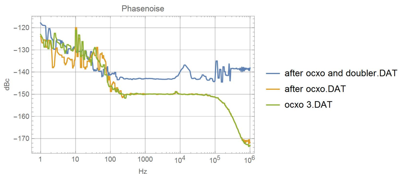
5mhz_to_10mhz_ocxo_again.pdf
